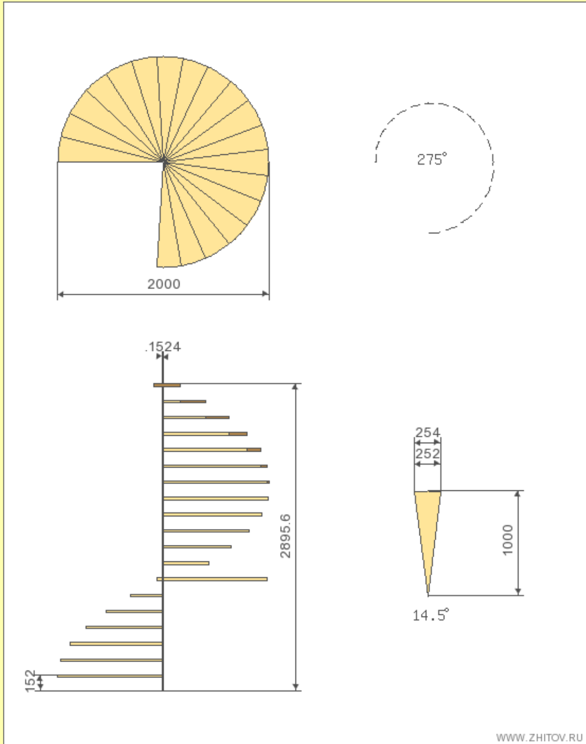
The total drawing a spiral staircase
